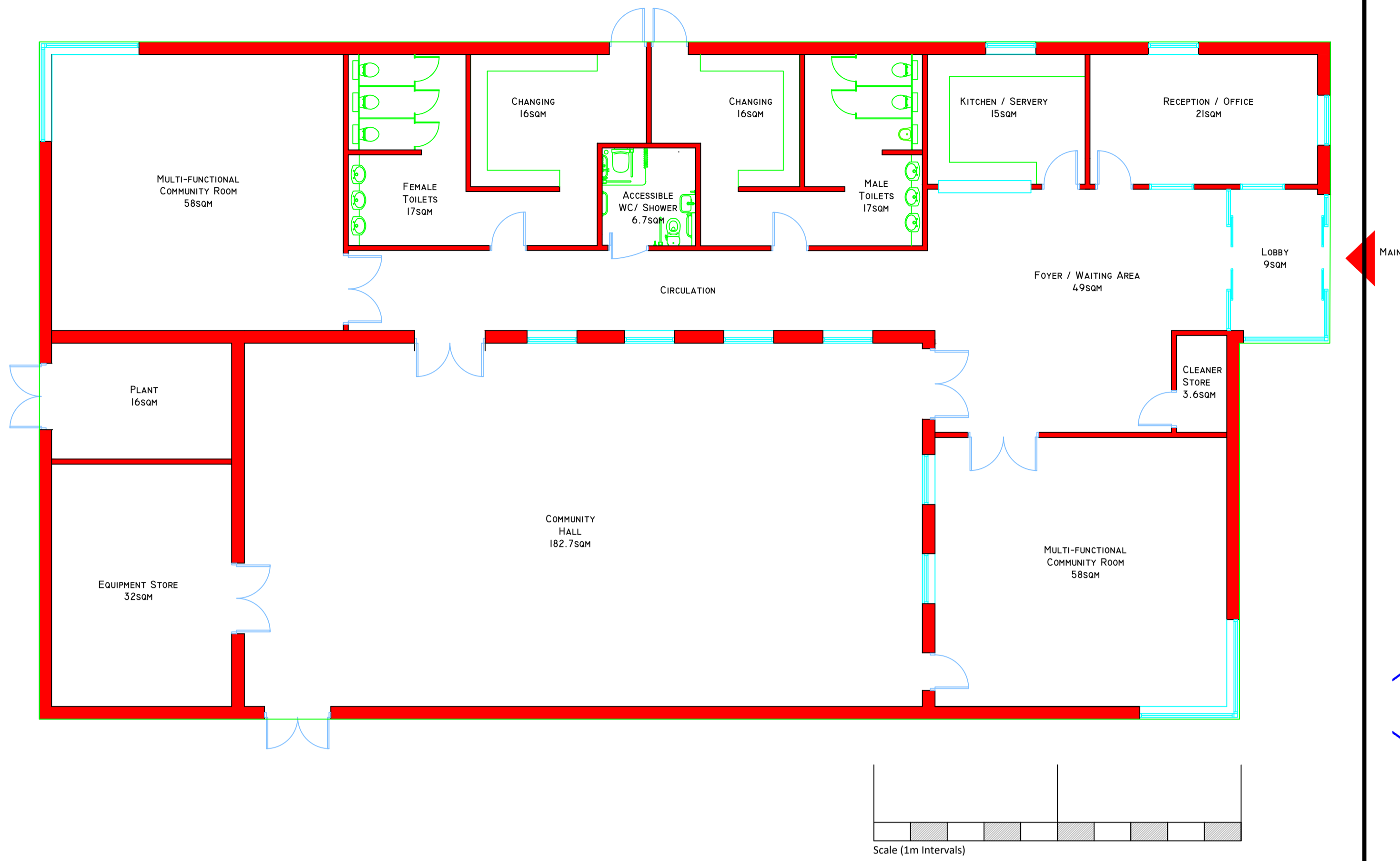
Suggested Layout 1 1:100
